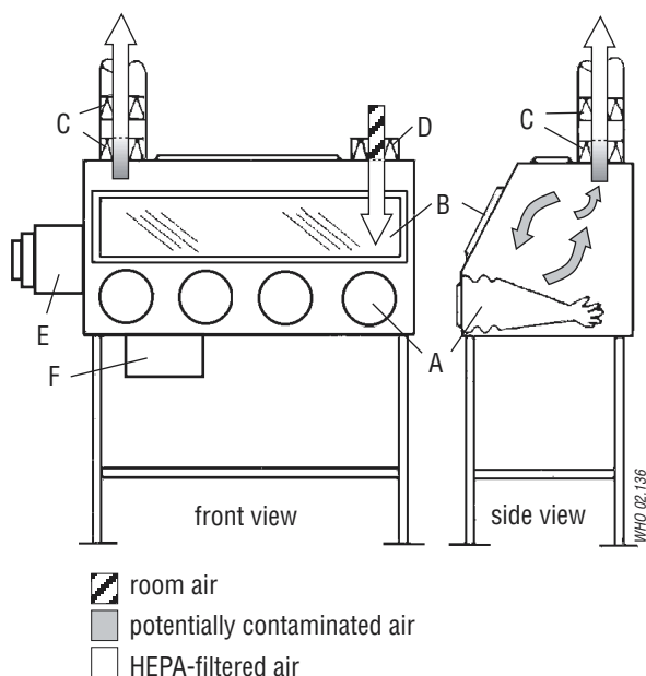
Figure 9. Schematic representation of a Class III biological safety cabinet (glove box).
